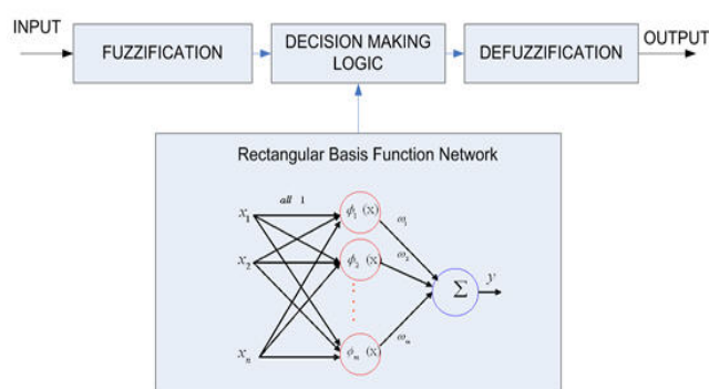
Fig. 1. The Fuzzy Graph Rectangular Basis Function Network diagram
