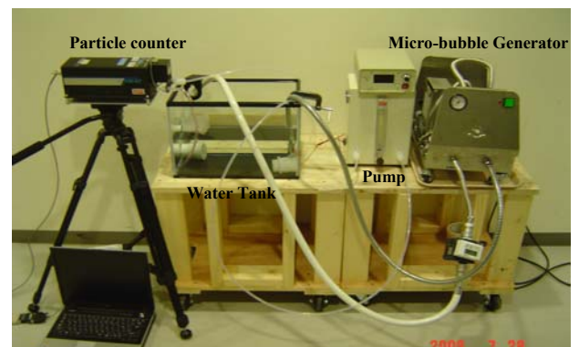
Fig. 1. Experimental apparatus
