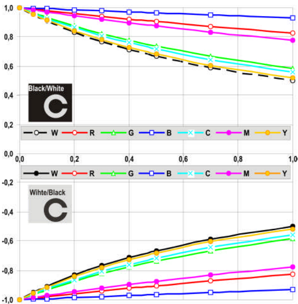
Fig. 3. Influence of different colour ambient light over colour luminance contrast for White task on Black background and Black task on White background
