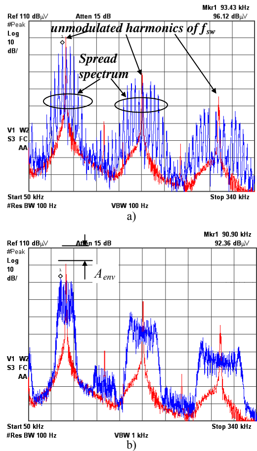
Fig. 3. Experimental power spectra of conducted EMI for unmodulated and modulated f_{sw} of PFC: (a) \Delta f_{sw} = 10 kHz , f_m = 5 kHz . (b) \Delta f_{sw} = 10 kHz , f_m = 1 kHz .
