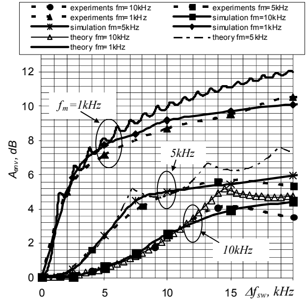
Fig. 4. Obtained attenuation A_{env} of EMI noise versus \Delta f_{sw} for different f_m resulting from the experiments, the simulations and FMT.
