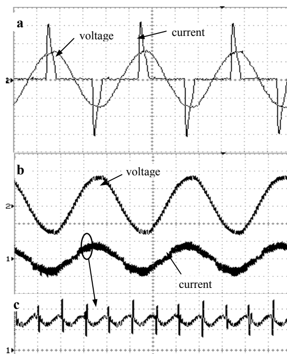
Fig. 1. Input current and voltage waveforms for resistive load of 100...110 W powered through TIS: a) directly and b) with PFC added. Scale: (a, b) current (1A/div; 5ms/div); voltage (200V/div; 5ms/div); (c) current (500mA/div; 10µs/div)
