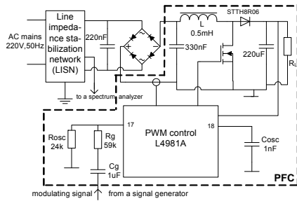
Fig. 2. Simplified schematic diagram of the experimental setup
