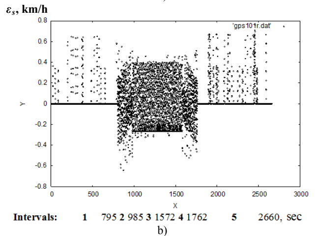
Fig. 5. Current values for: a) radial error (meters) and b) velocity error (km/h) for the receiver Graymark GPS-101 when the object is moving along the meridian with velocity profile 180 km/h (SHIFT=20)
