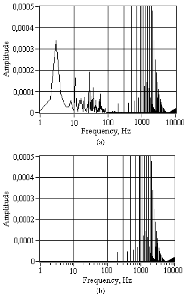
Fig. 4 Magnitude spectrum of pseudo-periodic test signal and low-frequency internal noise (a) and magnitude spectrum of frequency “fork” digital filter output (b) after blocking 16 spectral blocks
