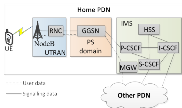
Fig. 1. Simplified UMTS network architecture to provide services over IMS
