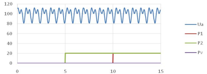
Fig. 5. Loading conditions that were simulated – arterial pressure U_a , external pressures P_1 and P_2 and venous pressure P_v .
