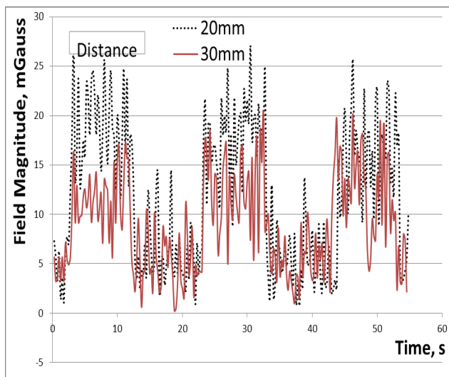
Fig. 12. Two parallel wire for LED supply magnetic field magnitude, current 0.3 A, distance 20 mm and 30 mm from sensor
