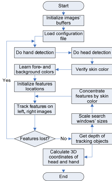
Fig. 1 Flow chart diagram of our proposed hand pointing system
